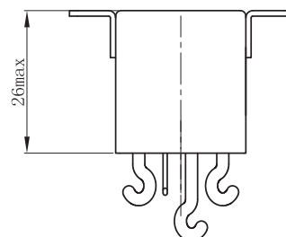
Mounting Code "8"
