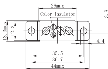
Mounting Code "3"
