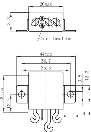
Mounting Code "3"
