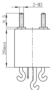
Mounting Code "0"
