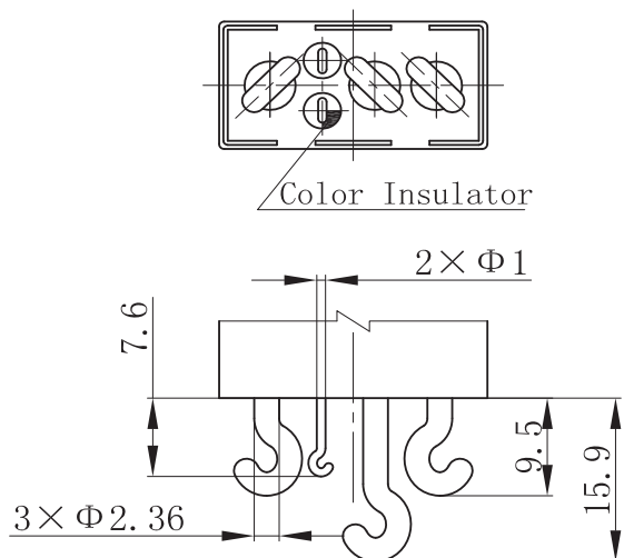
Pin Form “4”
