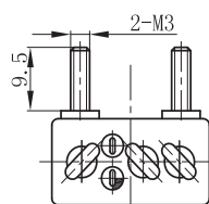
Mounting Code "2"
