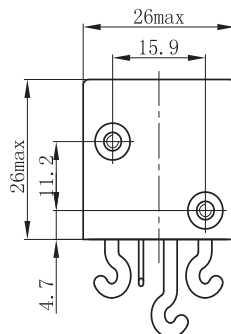
Mounting Code "5"
