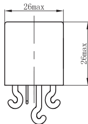
Mounting Code "0"
