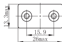
Mounting Code "4"
