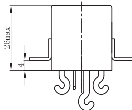
Mounting Code "2"
