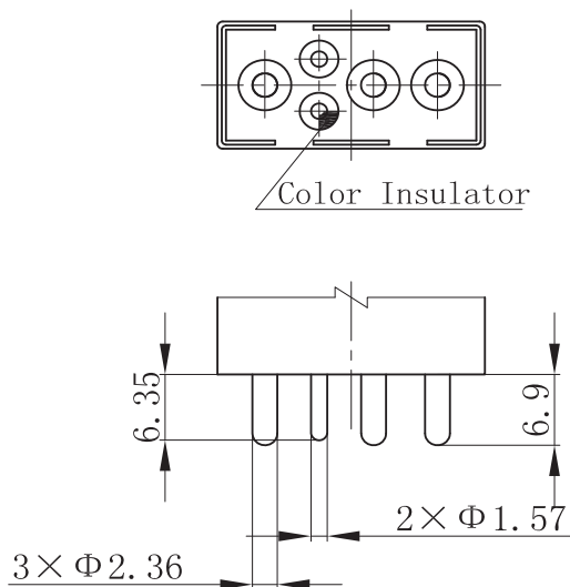
Pin Form “1”
