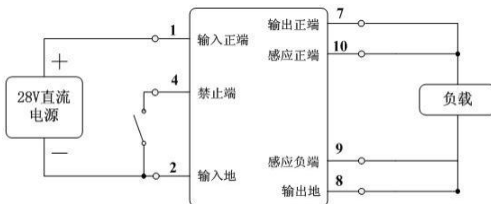
Figure 8. BSTHOL28 Series Product Usage Connection Diagram
