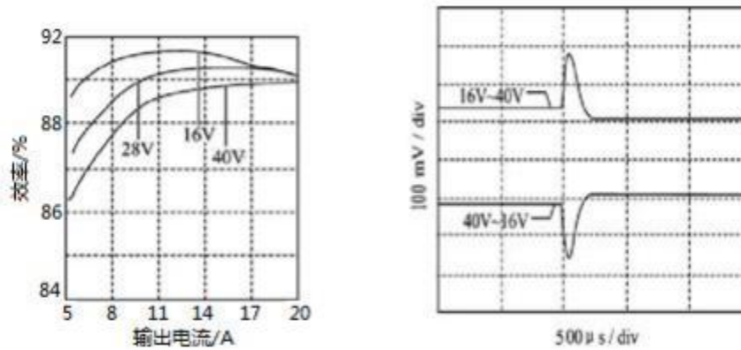
Figure 2. BSTHOL28 Efficiency Curve 3 BSTHOL28 Input Step Curve
