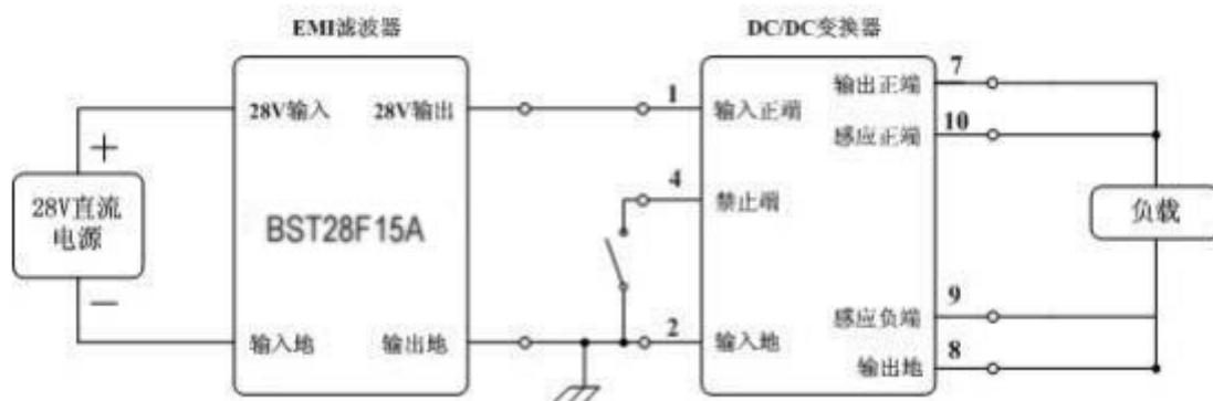
Figure 9. BSTHOL28 Series EMI Filter Connection Diagram
