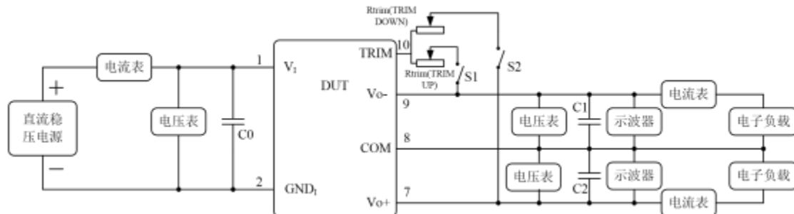
Fig 2. Schematic Diagram of Output Voltage Adjustment Test
