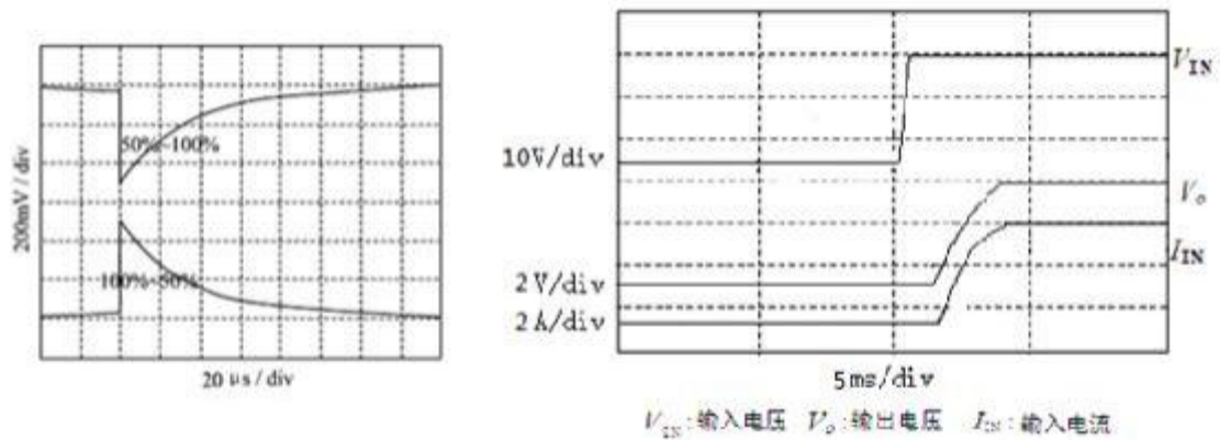
Figure 3. BSTHOL28 Load Step
