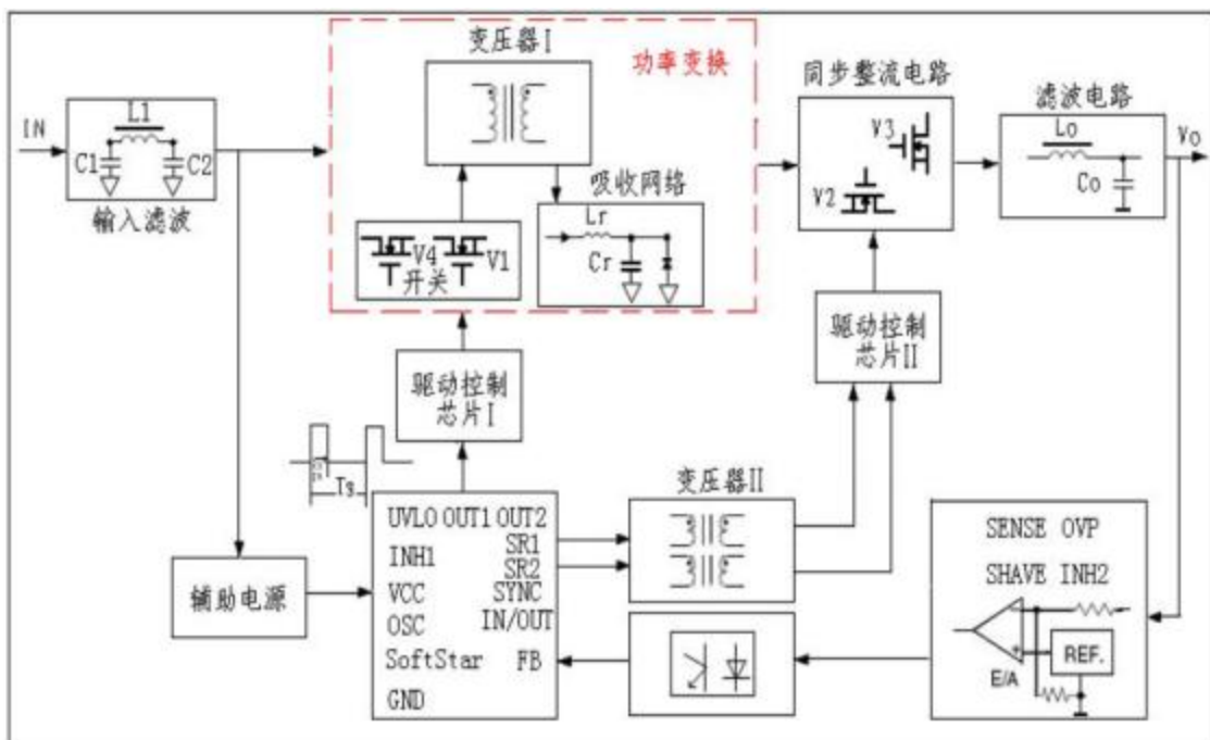
Figure 1. Block diagram of BSTHOL28S series circuit
