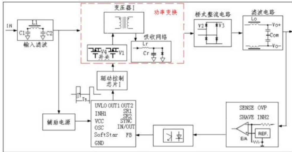
Figure 1. Block diagram of BSTHOL28 series circuit
