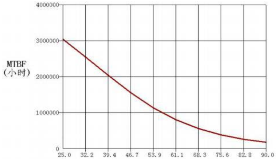
MTBF Temperature Profile (BSTHOL28)
