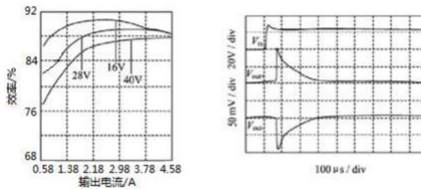
Figure 2. BSTHOL28 Efficiency
