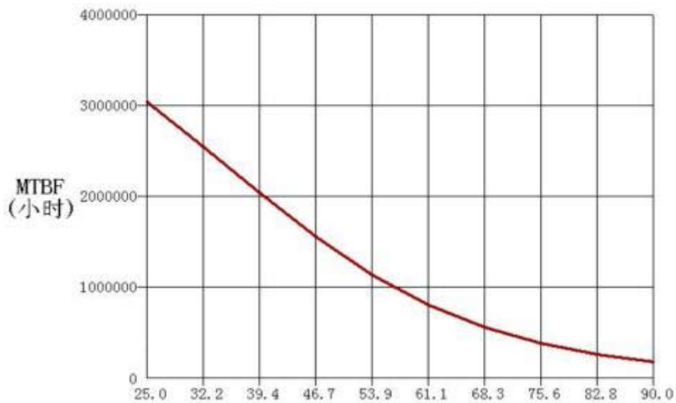
MTBF Temperature Profile (BSTHOL28)
