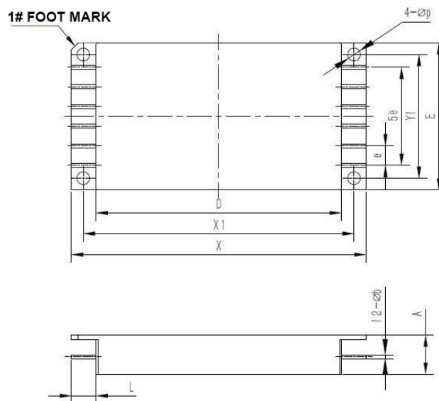
Figure 1. Dimensions
