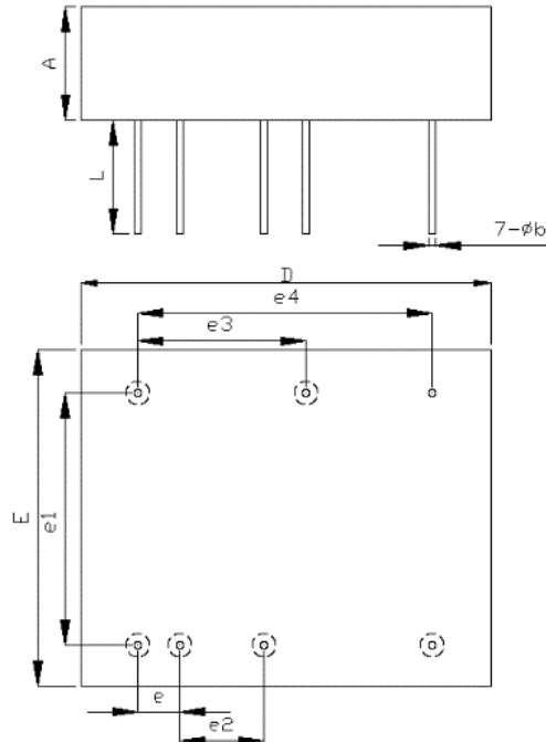
Figure 1. External dimensions of BSTCH28D15
