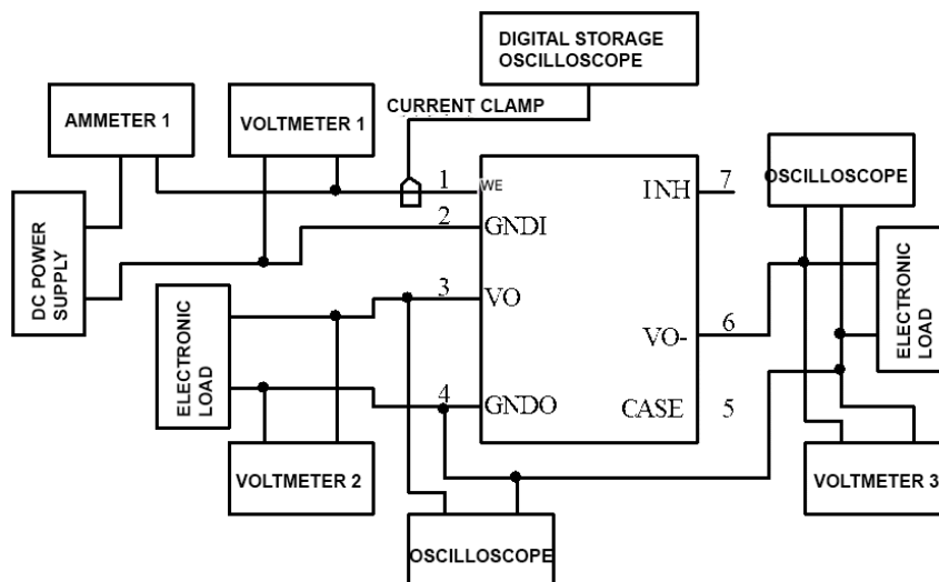
Figure 3. Test principle block diagram
