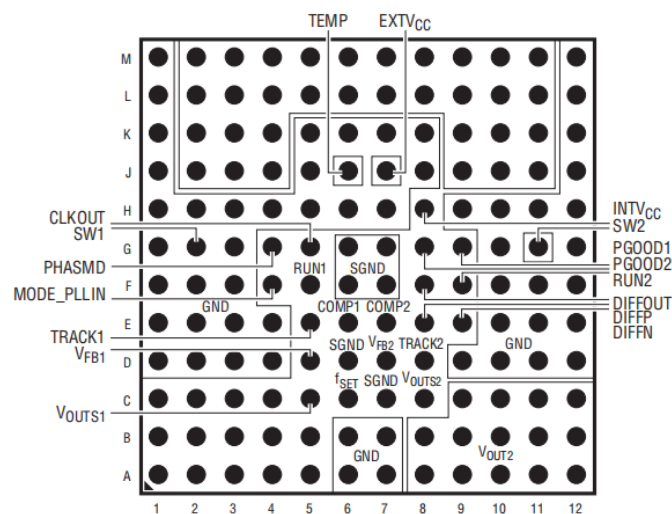
Figure 2BST4630 pinout
