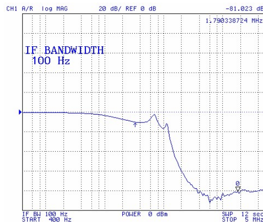
Figure 6. BST/ (20-50) -461-500 Insertion Loss
